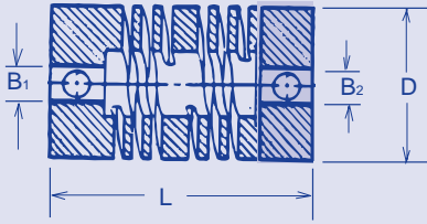
SET SCREW HUB TYPE NON RELIEVED
